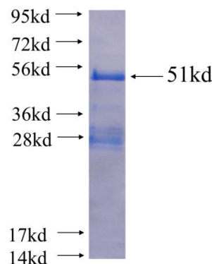
Recombinant human CUEDC2 SDS-PAGE
