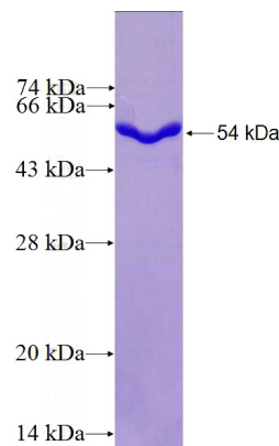
Recombinant Human USP8 SDS-PAGE
