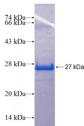
Recombinant Human EPN3 SDS-PAGE
