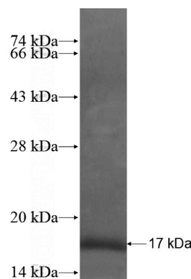
Recombinant Human NDUFA2 SDS-PAGE
