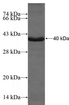
Recombinant Human DOCK1 SDS-PAGE
