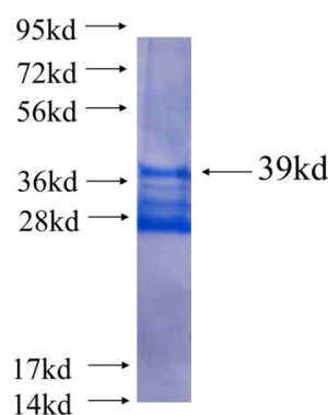
Recombinant human SLC22A15 SDS-PAGE
