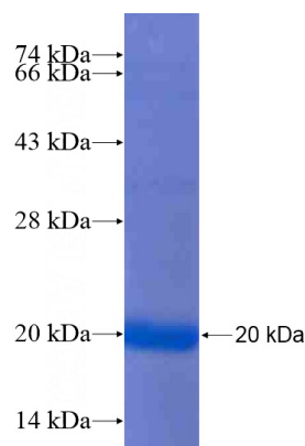
Recombinant Human PADI6 SDS-PAGE
