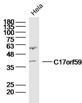
Fig1: Sample:HeLa Cell(Human) Lysate at 40 ug; Primary: Anti-C17orf59 at 1/300 dilution; Secondary: IRDye800CW Goat Anti-Rabbit IgG at 1/20000 dilution; Predicted band size: 37kD; Observed band size: 40kD
