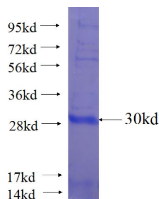
Recombinant human AID SDS-PAGE
