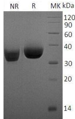
Human CD274/B7H1/PDCD1L1/PDCD1LG1/PDL1 (His tag) recombinant protein
