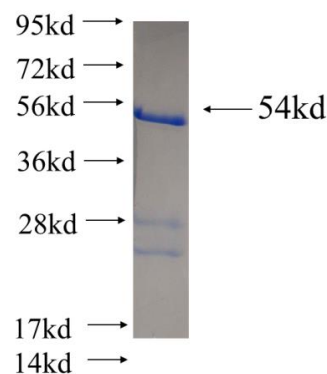
Recombinant human TPMT SDS-PAGE
