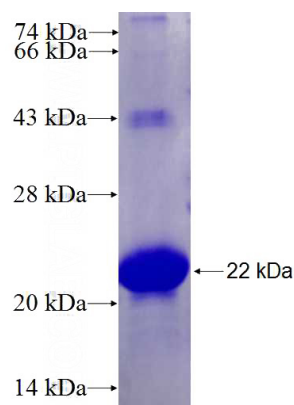
Recombinant Human RNF182 SDS-PAGE
