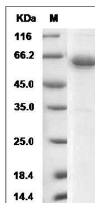
Rat JAM-2 / JAM-B Protein (Fc Tag) SDS-PAGE
