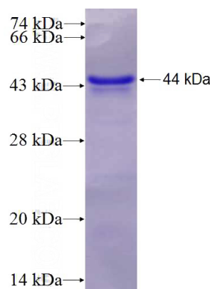
Recombinant Human CUL7 SDS-PAGE
