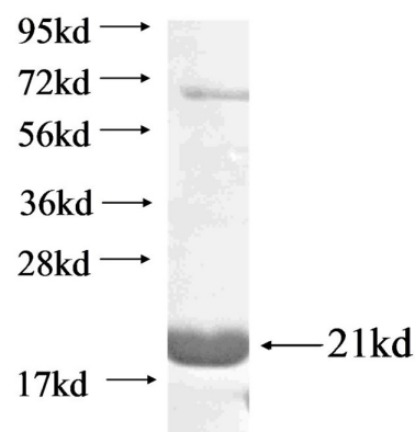
Recombinant Arabidopsis thaliana PFN2 SDS-PAGE
