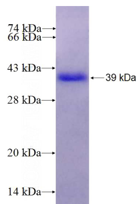
Recombinant Human PYGL SDS-PAGE
