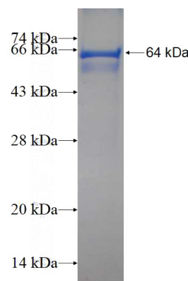
Recombinant Human AVIL SDS-PAGE
