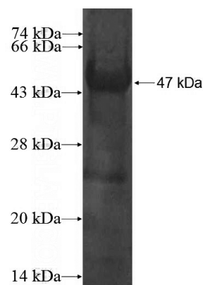
Recombinant Human JIP1 SDS-PAGE
