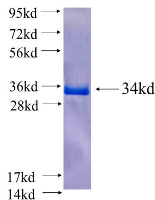
Recombinant human CPLX4 SDS-PAGE
