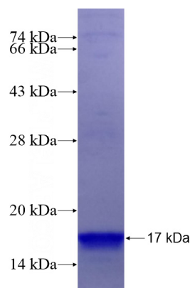
Recombinant Human CCL25 SDS-PAGE
