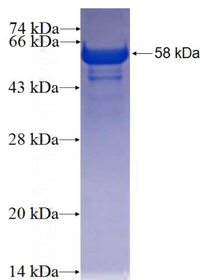
Recombinant Human ARHGAP28 SDS-PAGE
