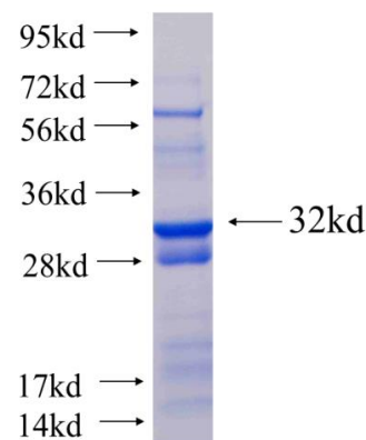
Recombinant human NDUFA9 SDS-PAGE
