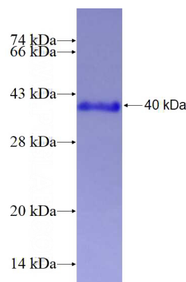
Recombinant Human SF3B14 SDS-PAGE
