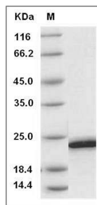
Human FGF19 Protein SDS-PAGE
