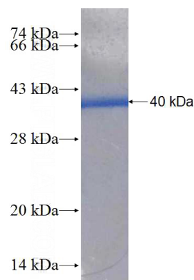
Recombinant Human GRIA1 SDS-PAGE
