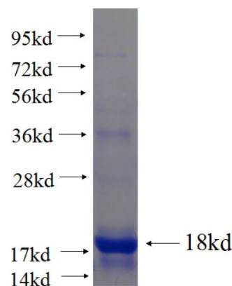
Recombinant human TNNI3 SDS-PAGE
