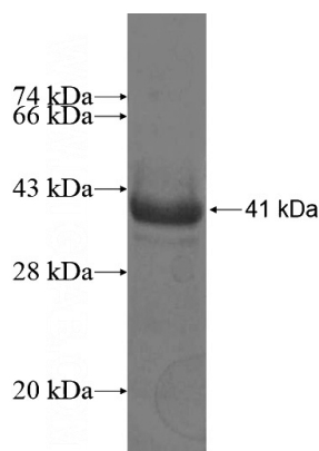
Recombinant Human CYP7A1 SDS-PAGE
