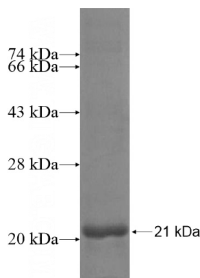
Recombinant Human GALNTL1 SDS-PAGE
