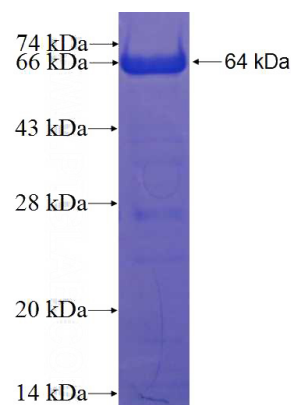
Recombinant Human C1orf113 SDS-PAGE
