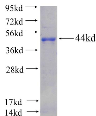
Recombinant human ZNF180 SDS-PAGE
