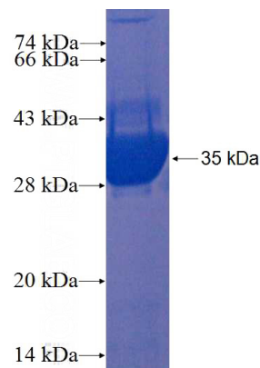
Recombinant Human DPH3 SDS-PAGE
