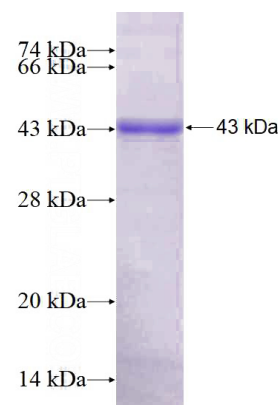
Recombinant Human TBX21,T-bet SDS-PAGE
