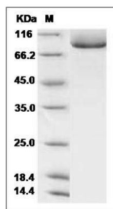
Human TGFBR3 / Betaglycan Protein (His Tag) SDS-PAGE
