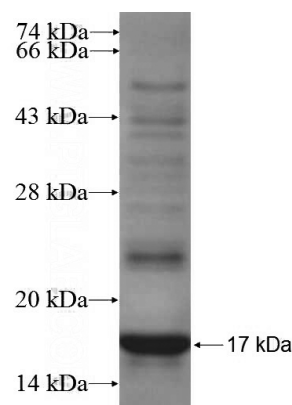
Recombinant Human TP73 SDS-PAGE
