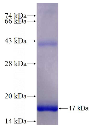
Recombinant Human NOX1 SDS-PAGE
