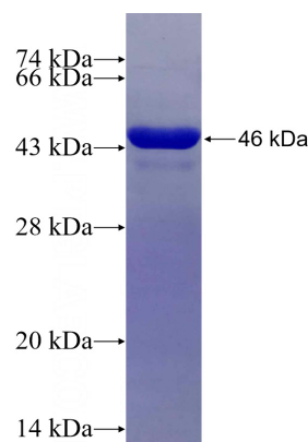
Recombinant Human RNF128 SDS-PAGE
