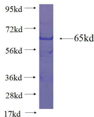
Recombinant human ASNA1 SDS-PAGE
