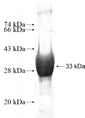
Recombinant Human GNPDA2 SDS-PAGE
