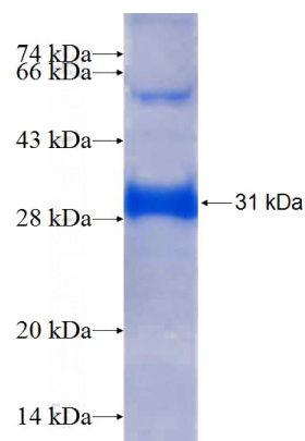
Recombinant Human PPM1J SDS-PAGE
