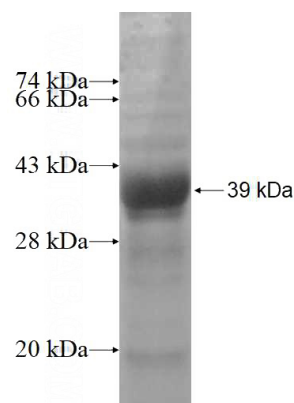
Recombinant Human ALLC SDS-PAGE
