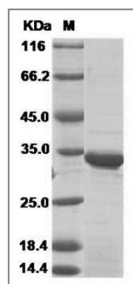
Human DHRS9 Protein (His Tag) SDS-PAGE
