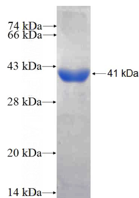
Recombinant Human LONP1 SDS-PAGE
