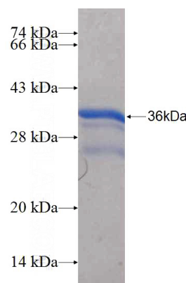
Recombinant Human Myogenin SDS-PAGE
