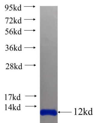
Recombinant human FLI1 SDS-PAGE
