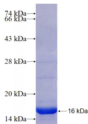
Recombinant Human TAGLN2 SDS-PAGE
