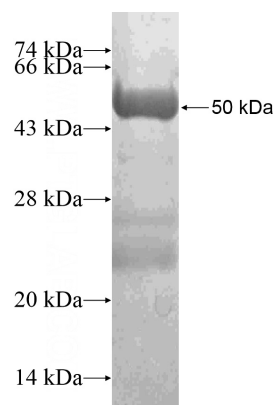
Recombinant Human A2BP1 SDS-PAGE
