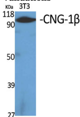
Fig1.; Western Blot analysis of various cells using CNGB-1β Polyclonal Antibody
