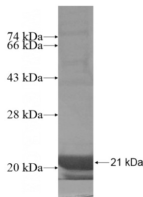
Recombinant Human TCL1B SDS-PAGE
