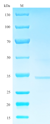
Recombinant Human ELN SDS-PAGE
