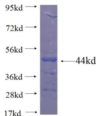
Recombinant human TBP SDS-PAGE
